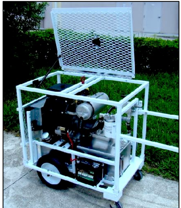
Economical & Productive 20”/24” Hydraulic Saw For Interior “Fume Free Saw”
