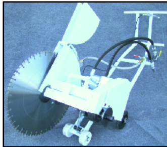
Economical & Productive 20”/24” Hydraulic Saw For Interior “Fume Free Saw”
